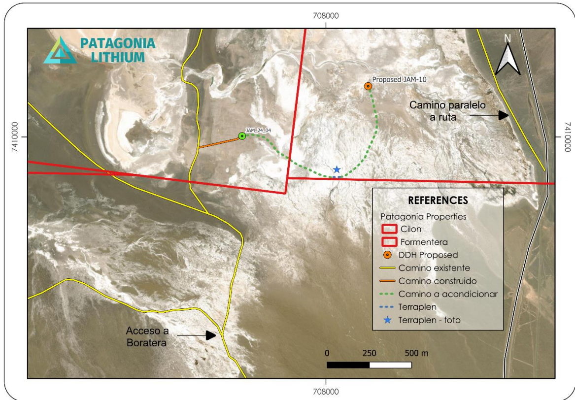
Figure 3. Map location of well four - labelled JAM-10
