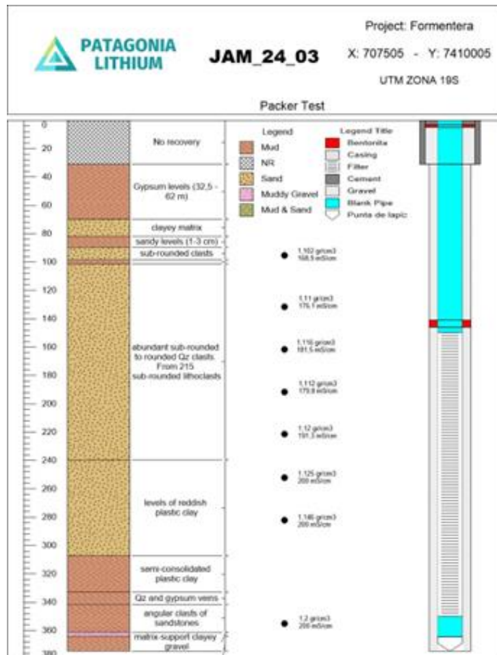
Figure 2. Shows core lithology, well design and wet sands at 90m depth and quartz gravel at 340m.
