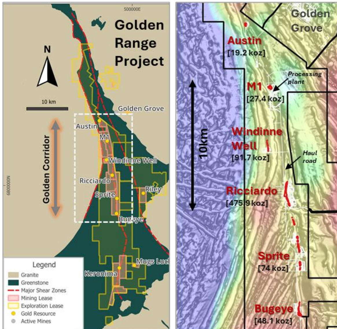
Figure 2: The 'Golden Corridor' within the Golden Range Project. The image on the right is gravity over shaded residual magnetic RTP.
